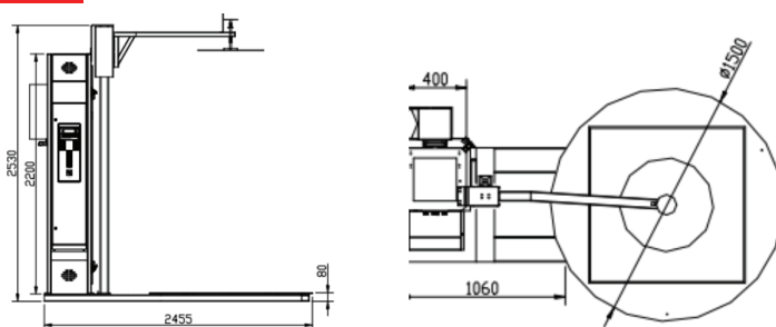
Pre-stretch film carriage
